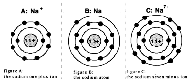
Figure 1: three chemical species
